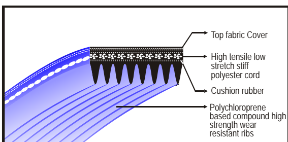
Ribbed Belts
